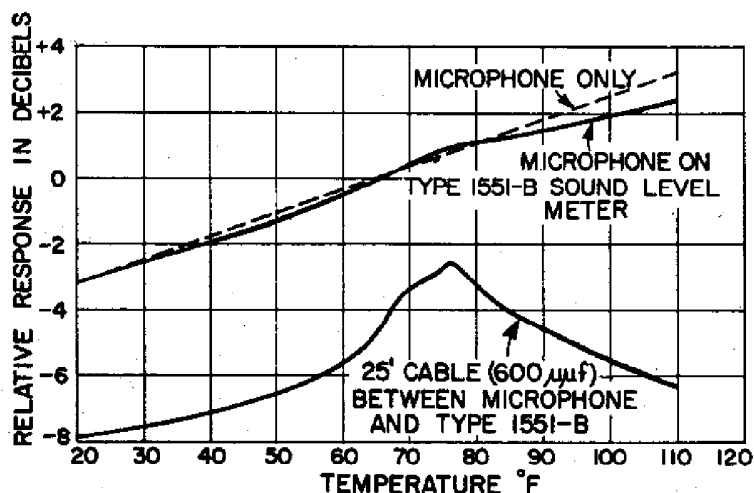
Figure 3. Variation in Response as a Function of Temperature for Type 1560-P1 Microphone. (Curves are shown for: open-circuit output voltage of microphone; microphone output to Sound-Level Meter (no cable); and microphone output to Sound-Level Meter with 25-ft extension cable (Type 1560-P73).
